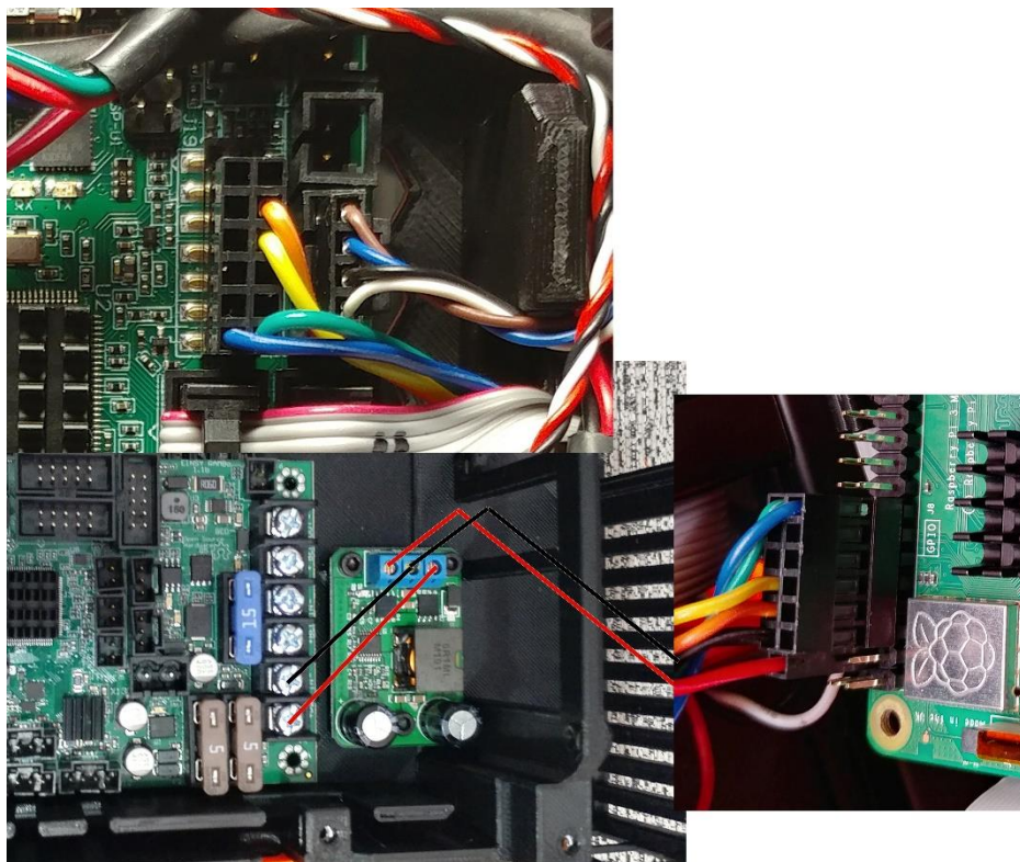
Emsy board connections
